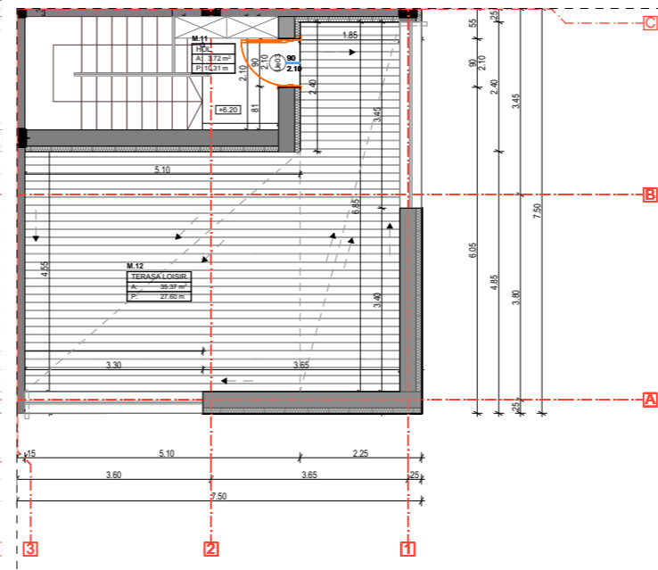
PLAN MANSARDA
