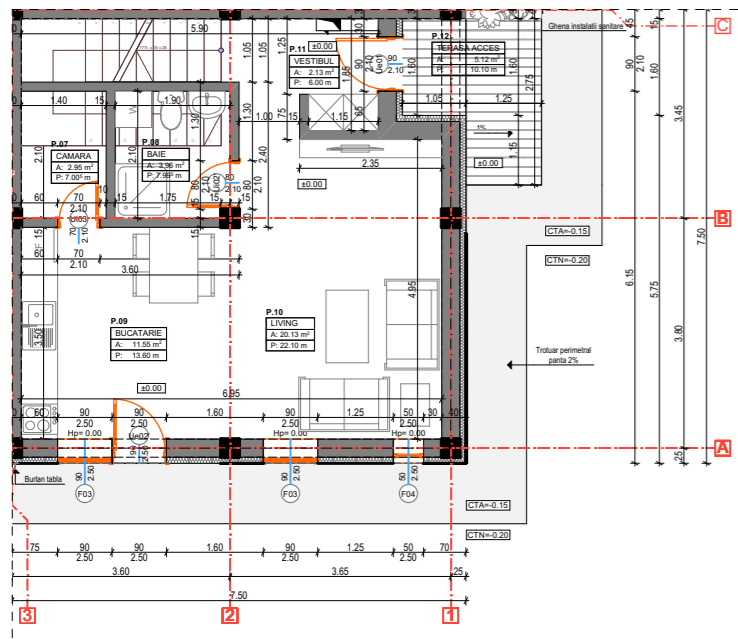
PLAN PARTER
