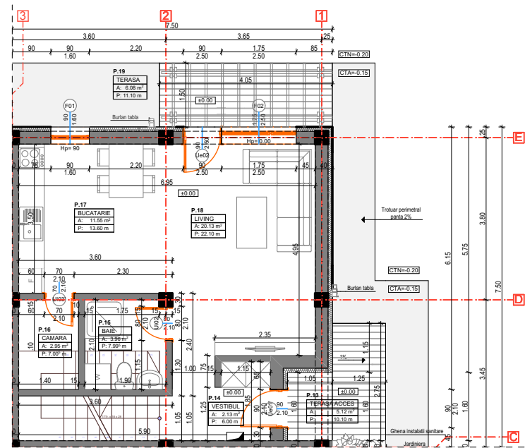
PLAN PARTER
