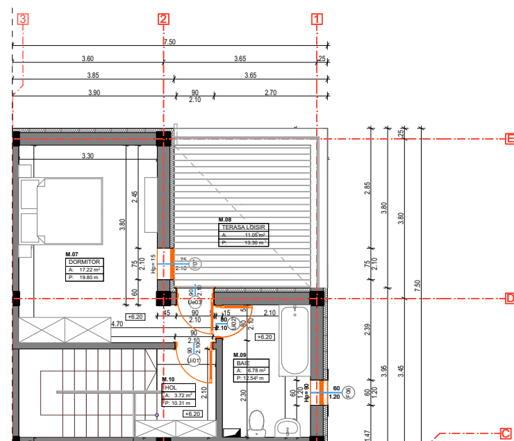
PLAN MANSARDA
