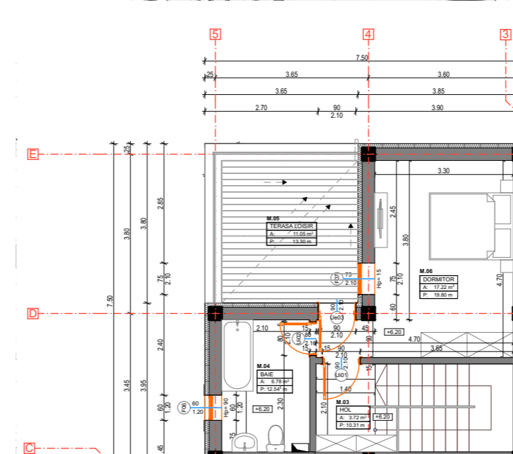
PLAN MANSARDA
