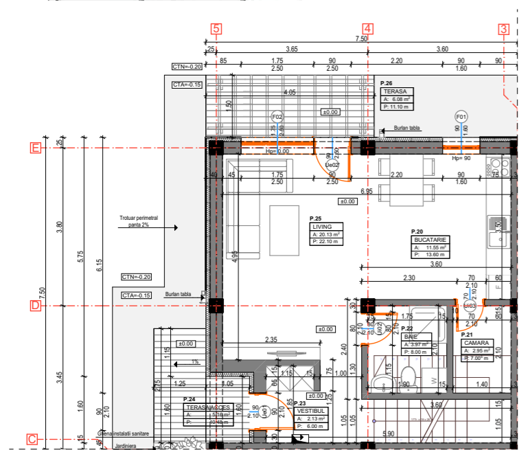
PLAN PARTER
